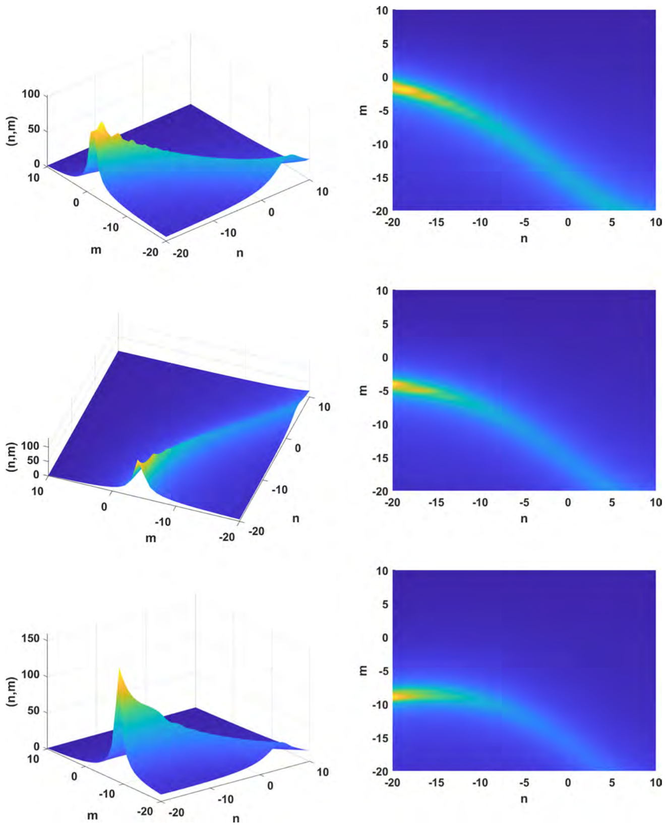
Fig. 1 Grammian \hat{\alpha}_{n,m} : for numerical values \eta = 0.8 - 0.54i , \zeta = 4.5 + 0.25i , q = 3 , b = 2
