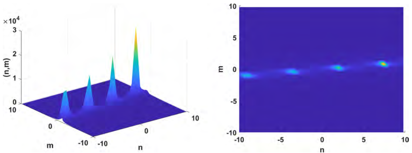
Fig. 5 Discrete breather: for numerical values \eta = 5.9 + 0.54i , q = 0.9 , b = 0.6
