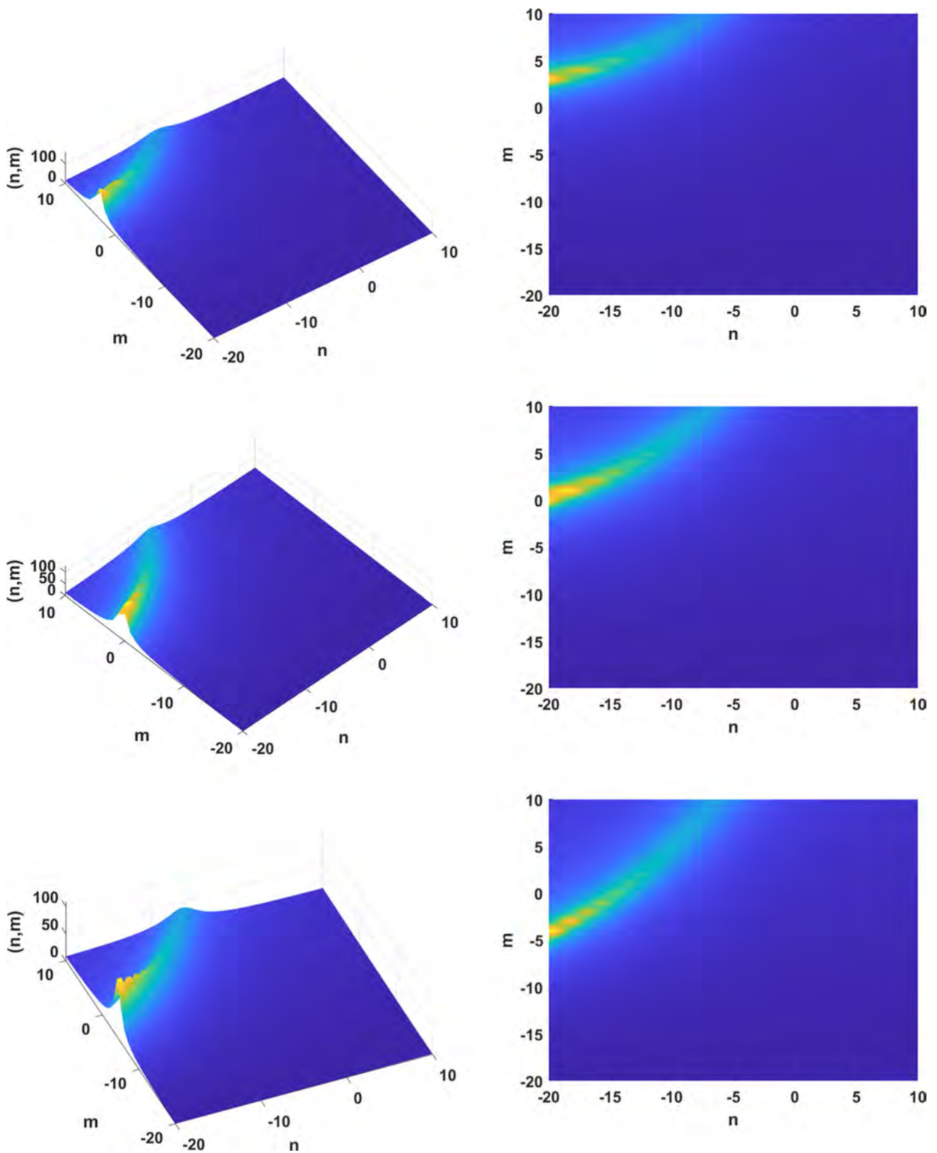
Fig. 2 Gramian \hat{\beta}_{n,m} for numerical values \eta = 0.8 + 0.54i , \zeta = 4.1 - 0.45i , q = 3 , b = 2
