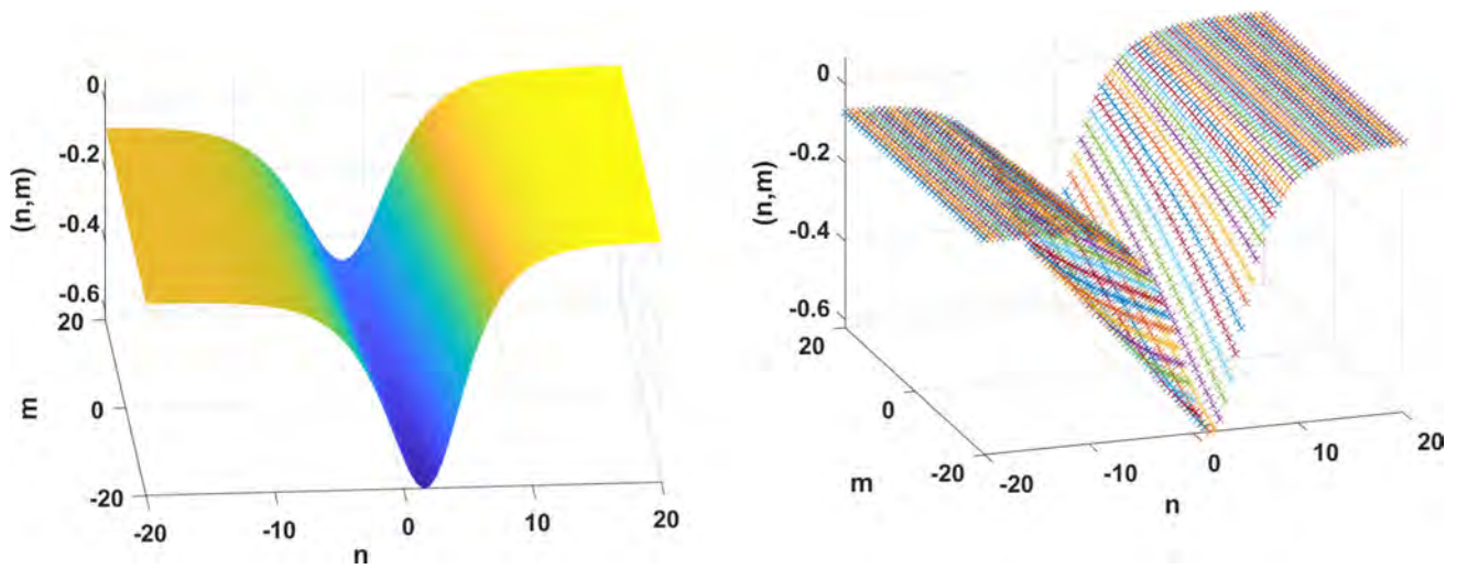
Fig. 4 Dark soliton: for numerical values \eta = 0.8 + 0.53i , q = 3 , b = 2
