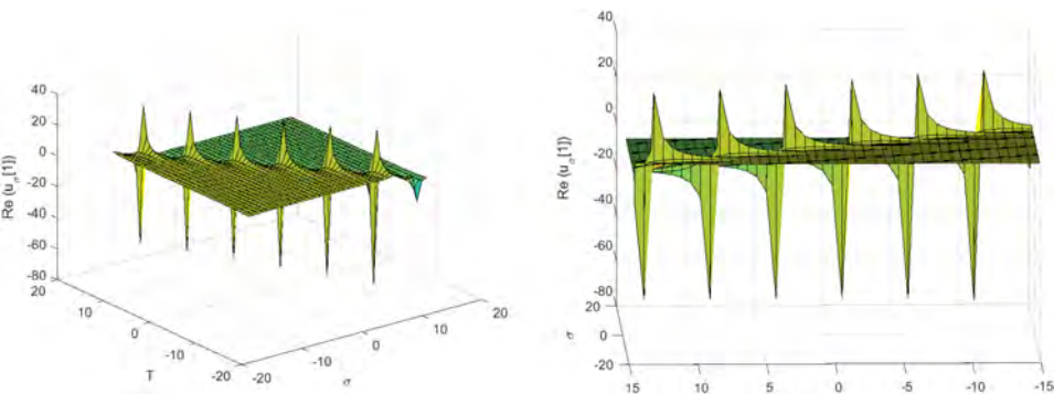
Fig. 6. Dynamics of peak solutions: for numerical values \lambda = 1.9 , a = 3 .
