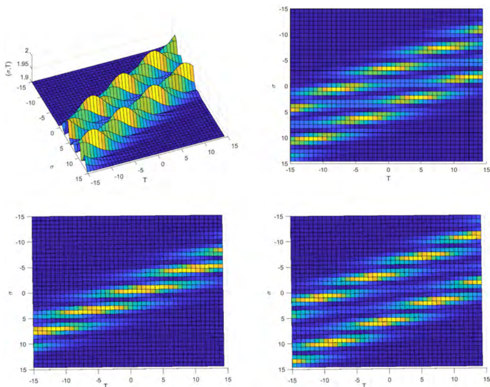
Fig. 1. Dynamics of \hat{N}_{\sigma,11} = \hat{N}_{\sigma,22} : for numerical values \lambda = 1.9 + 0.71i , \mu = 1.8 + 0.5i , a = 2 Parallel traveling of two double breathers, interaction and after interaction.
