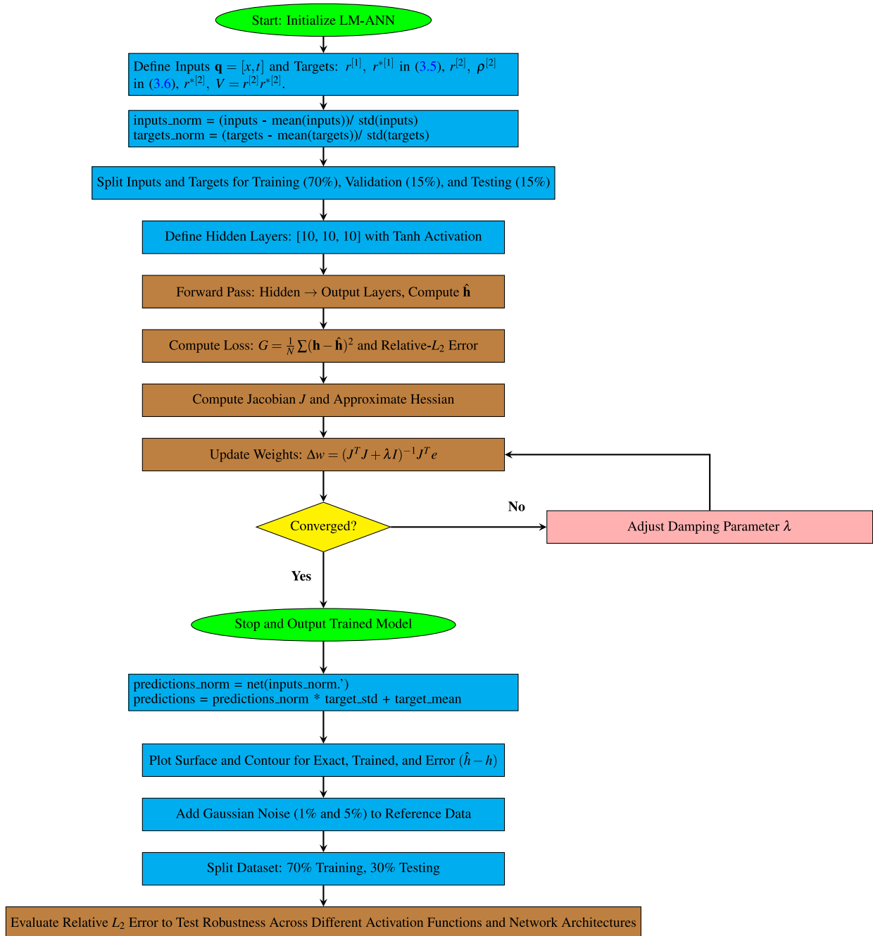
Fig. 1. Flowchart of the LM-ANN framework.
