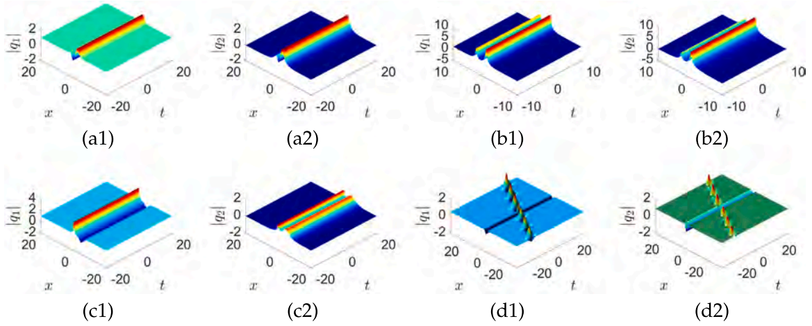
Fig. 4. (a1) and (a2): One parallel dark-bright and one parallel bright-bright soliton solutions by taking \mathbf{q}_- = (1, 0)^T , \sigma = 10^{-3} , K_6 = 0.5 , \kappa_5 = \chi_6 = 1 , \kappa_6 = e^{\frac{2}{10} + \frac{3}{5}i} , \alpha_5 = \alpha_6 = \frac{1}{2}\pi , k = 1 . (b1) and (b2): Two parallel bright-bright soliton solutions by taking \mathbf{q}_- = (1, 0)^T , \sigma = 10^{-3} , K_6 = 0.5 , \kappa_5 = e^{2-2i} , \kappa_6 = e^{\frac{3}{5} - \frac{6}{5}i} , \chi_6 = 1.5 , \alpha_5 = \alpha_6 = \frac{1}{2}\pi , k = 0 . (c1) and (c2): One parallel bright-bright and one parallel dark-bright soliton solutions by taking \mathbf{q}_- = (1, 0)^T , \sigma = 10^{-3} , K_6 = 0.5 , \kappa_5 = e^{\frac{2}{10} + \frac{3}{5}i} , \kappa_6 = 2.8 , \chi_6 = -0.2 , \alpha_5 = \alpha_6 = \frac{1}{2}\pi , k = 0 . (d1) and (d2): One dark-dark and one breather-breather soliton solutions by taking \mathbf{q}_- = (\frac{1}{2}e^{-\frac{1}{10}i\pi}, -\frac{\sqrt{3}}{2}e^{-\frac{1}{10}i\pi})^T , \sigma = 10^{-3} , K_6 = 0.98 , \kappa_5 = \chi_6 = 1 , \kappa_6 = 0.5 , \alpha_5 = \frac{1}{2}\pi , \alpha_6 = \frac{4}{5}\pi , k = 1 .
