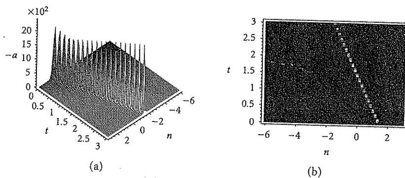
Figure 3.4. 3D and density plots of a_n .
