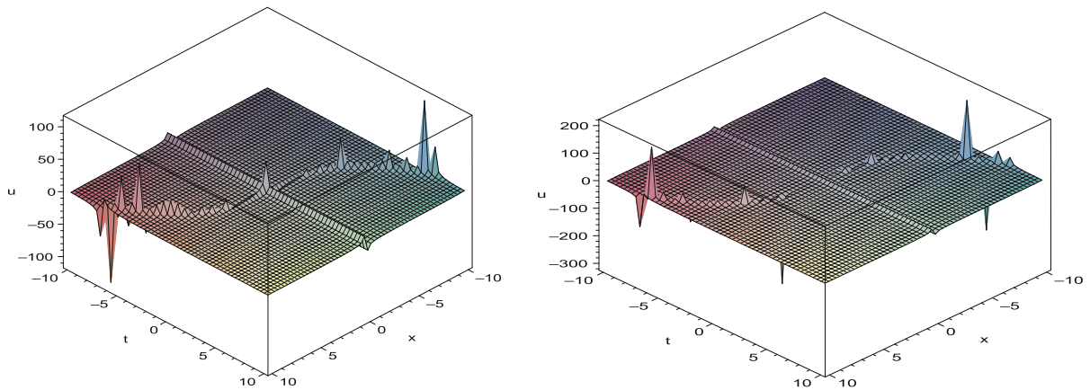
Fig. 2. Pictures of the solution (3.14) with c = 0 (left) and c = 2 (right).
