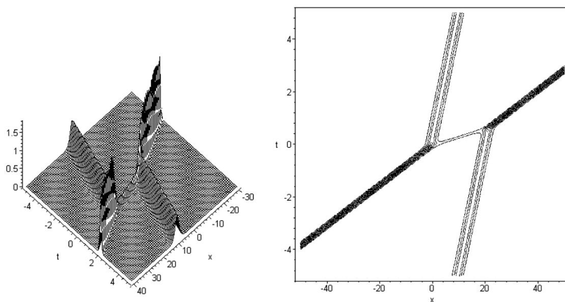
Fig. 5. The plot of two solitons splitting into three solitons and then fusing into two solitons to the new coupled higher-order Ito equation. The parameters used are a_1 = \frac{p_2}{p_1} + 10^{-10} , b_2 = \frac{a_2 p_2^2 b_1}{p_1^2} , p_1 = 1.9 , p_2 = 1.2 , a_2 = 2 , b_1 = 1 , b_2 = 3 , y = 0 . The left figure shows a three-dimensional plot and the right figure shows a contour map.
